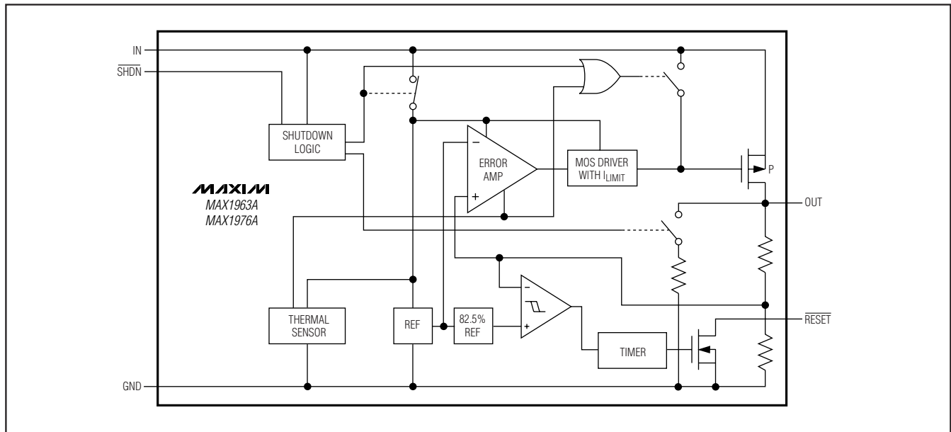
Figure 1. Functional Diagram
