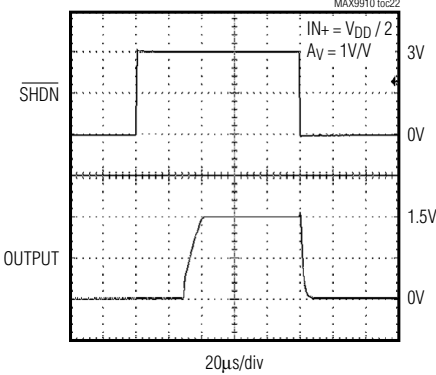
SHUTDOWN RESPONSE
