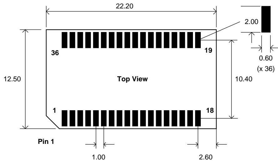
Figure 58. Recommended PCB Pad Sizes
