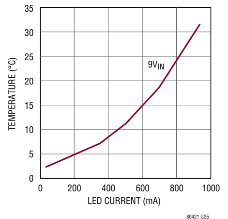
Junction Temperature Rise vs Load, Boost Operation, 18.1V at 1A LED String
