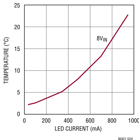
Junction Temperature Rise vs Load, Boost Operation, 13.6V at 1A LED String
