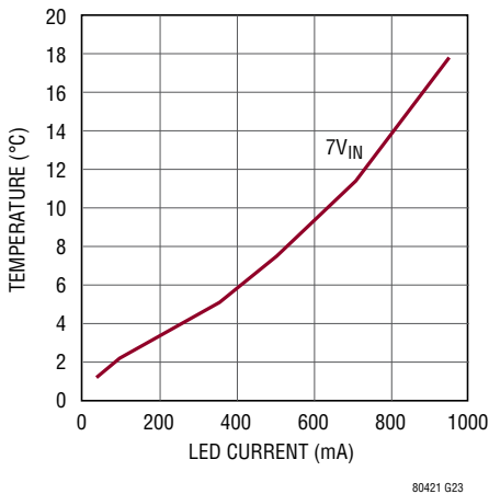
Junction Temperature Rise vs Load, Boost Operation, 10.9V at 1A LED String
