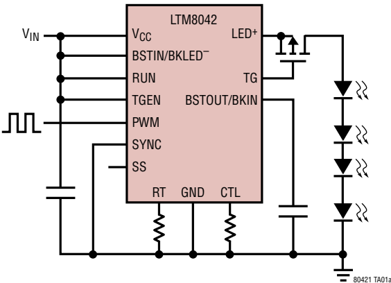
Figure 1. The LTM8042/LTM8042-1 Can Control a P-Channel PWM Switch
