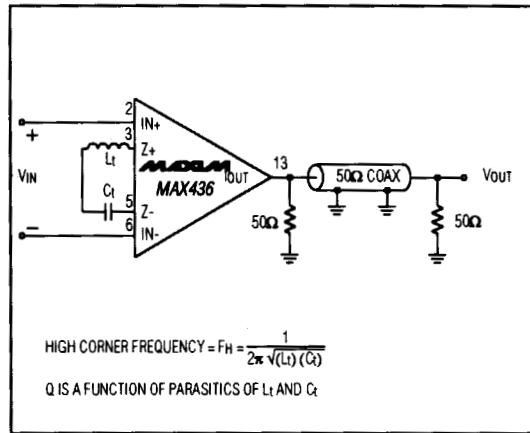
Figure 14. Tuned Amplifier
