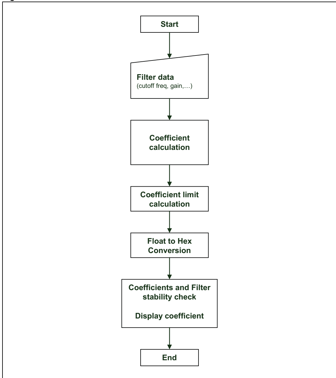
Figure 10. Code structure
