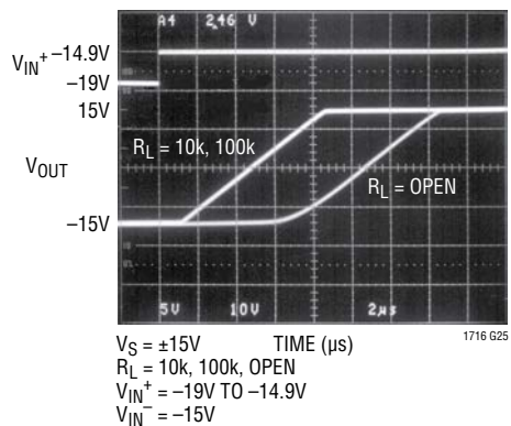
Below V_S^- Fault (Rising)
