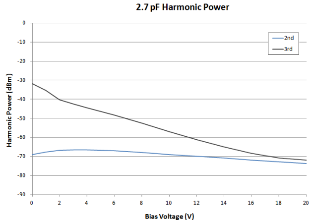
Figure 2. Harmonic Power
