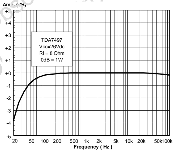
Figure 4. Frequency Response
