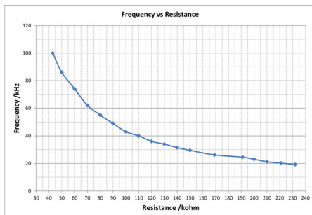
Figure 4 Frequency Versus R_{FREO}
