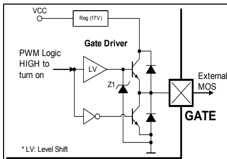
Figure 15 Gate Driver
