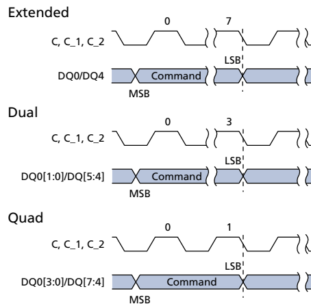
Figure 41: PROGRAM/ERASE SUSPEND or RESUME Timing
