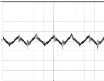
Output voltage ripple at: T_{ref} = +25^{\circ}\text{C} , V_i = 53\text{ V} , I_o = 60\text{ A} resistive load. Trace: output voltage (100mV/div.). Time scale: (2 μs/div.).
