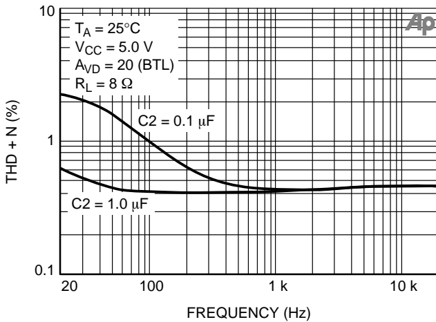
Figure 6. THD + N vs. Frequency (PL = 500 mW)
