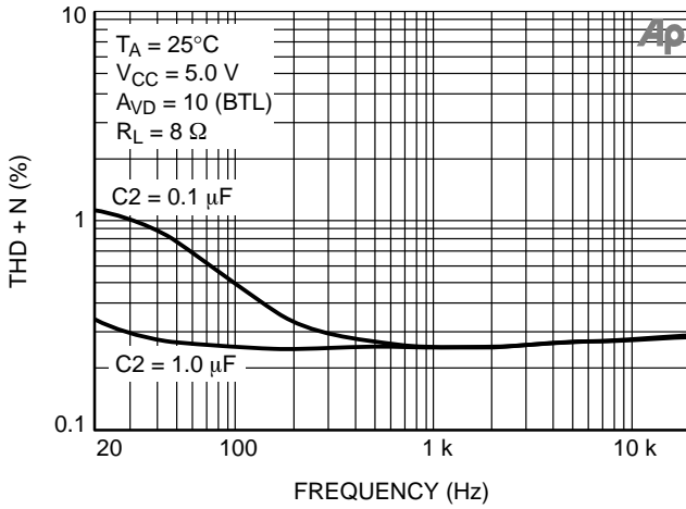
Figure 4. THD + N vs. Frequency (PL = 500 mW)
