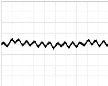
Output voltage ripple (5 mV/div.) at: T_{ref} = +25^\circ\text{C} , I_O = 60 A electrical load, V_I = 3.3 V. Time scale: 5 μs/div. Output capacitor: 660 μF electrolysis type. See the filter in the Output ripple and noise section (EMC Specification).
