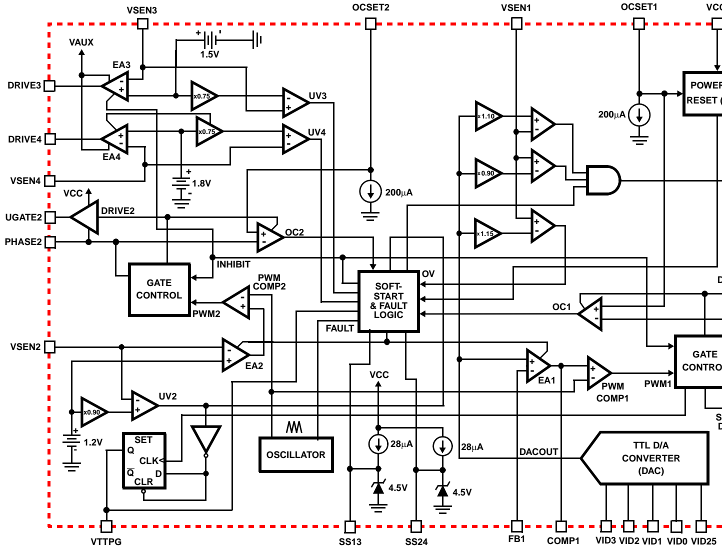
FIGURE 1. BLOCK DIAGRAM
