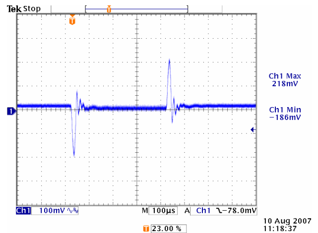
Figure 13. Vin=12V, Vout=2.5V
