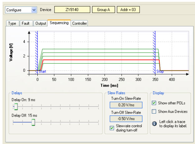
Figure 22. POL Configure Sequencing Window
