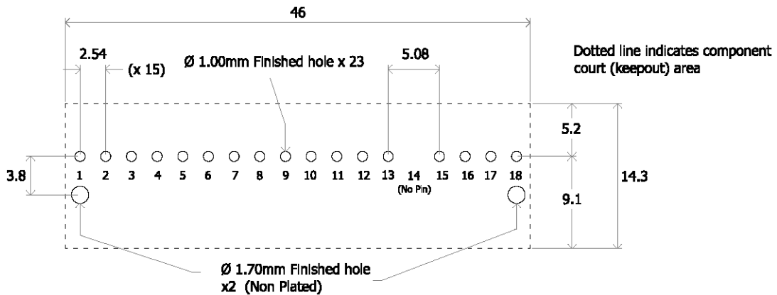
Figure 47. Mechanical Drawing
