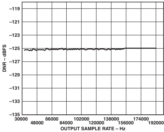
TPC 33. DNR (Unweighted) vs. Output Sample Rate, f_{S\_IN} = 48 kHz, -60 dBFS 1 kHz Tone
