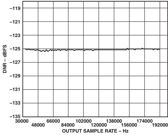
TPC 31. DNR (Unweighted) vs. Output Sample Rate, f_{S\_IN} = 96 kHz, -60 dBFS 1 kHz Tone
