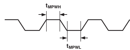
Figure 3. MCLK_IN Timing
