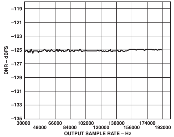
TPC 34. DNR (Unweighted) vs. Output Sample Rate, f_{S\_IN} = 44.1 kHz, -60 dBFS 1 kHz Tone
