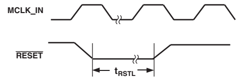
Figure 2. RESET Timing
