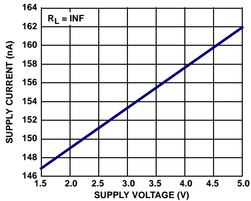
FIGURE 1. ISL28196 SUPPLY CURRENT vs SUPPLY VOLTAGE
