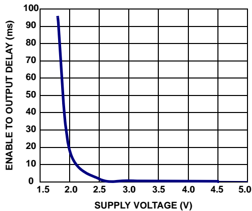
FIGURE 15. ISL28196 ENABLE TO OUTPUT DELAY TIME vs SUPPLY VOLTAGE
