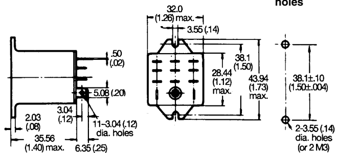
Mounting holes
