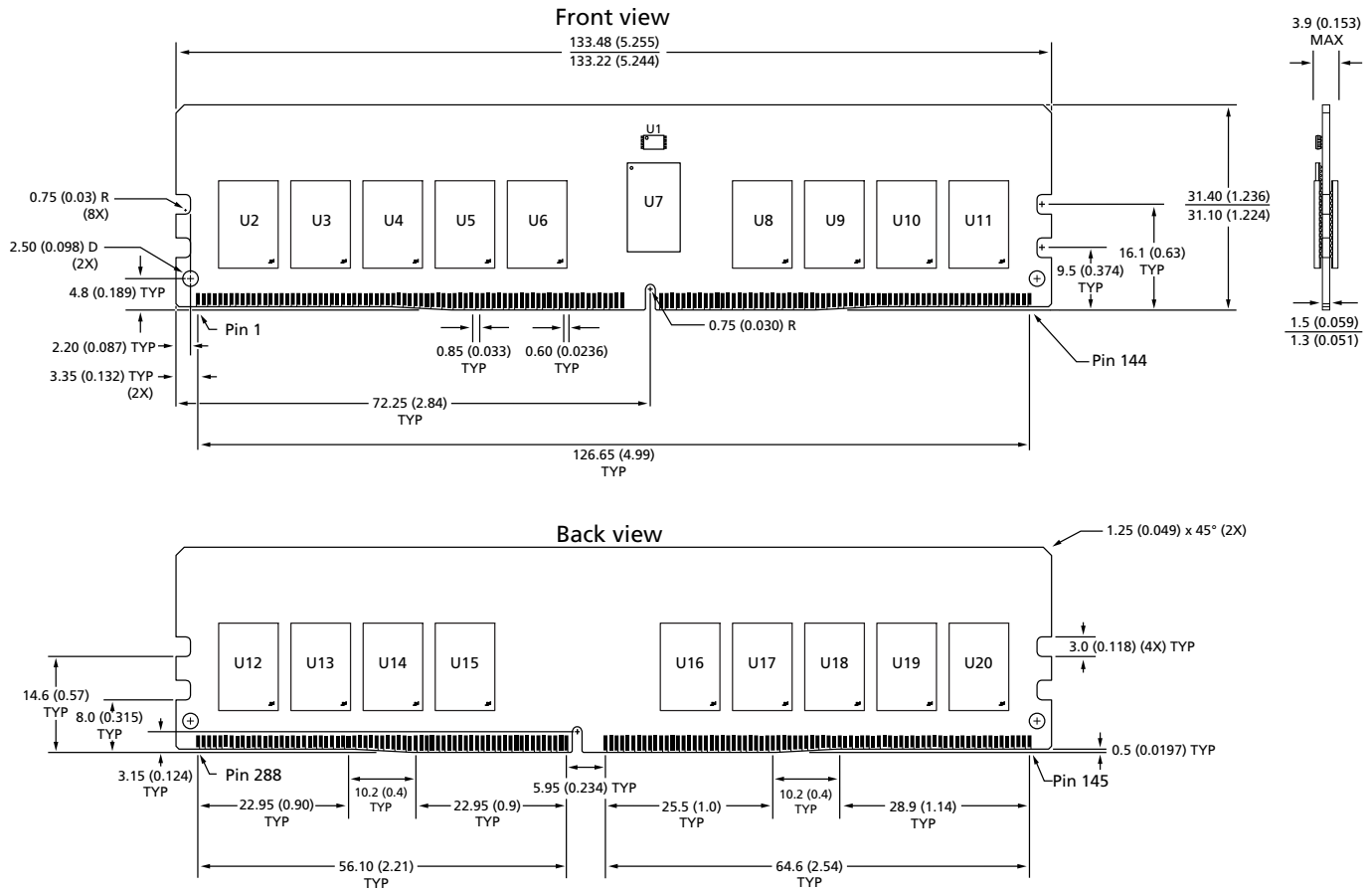
Figure 3: 288-Pin DDR4 RDIMM (R/C-C1, R/C-C2)
