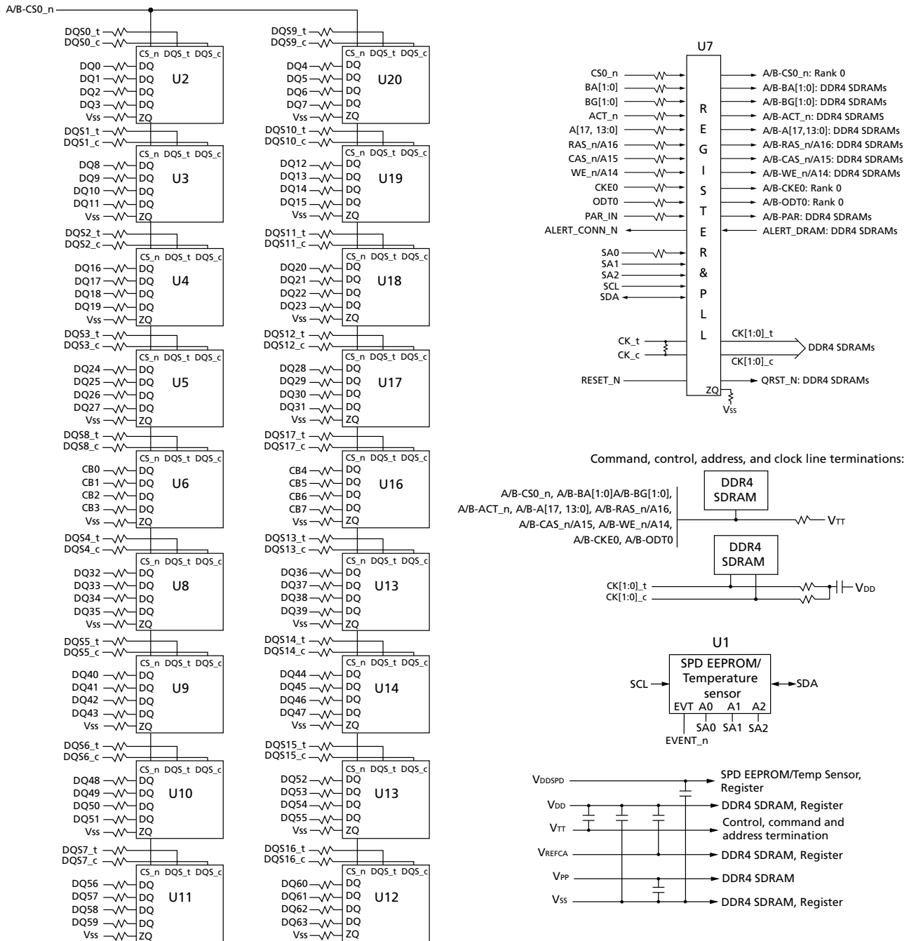
Figure 2: Functional Block Diagram (R/C-C1, R/C-C2)
