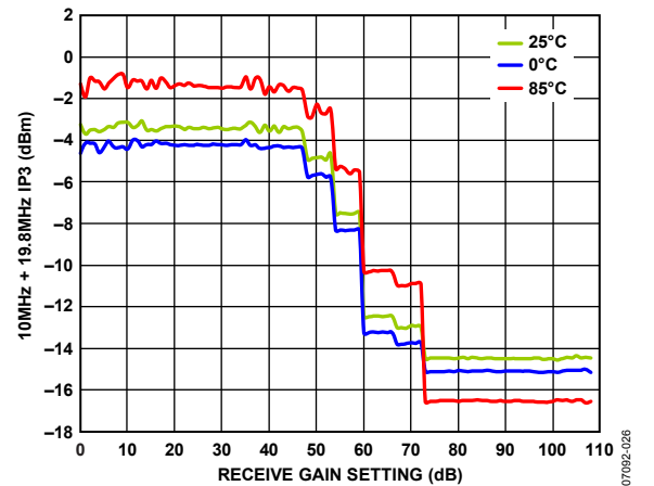
Figure 34. RXHB1RF Receive IP3, 10 MHz + 19.8 MHz vs. Gain Setting
