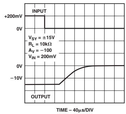
TPC 27. Negative Overvoltage Recovery
