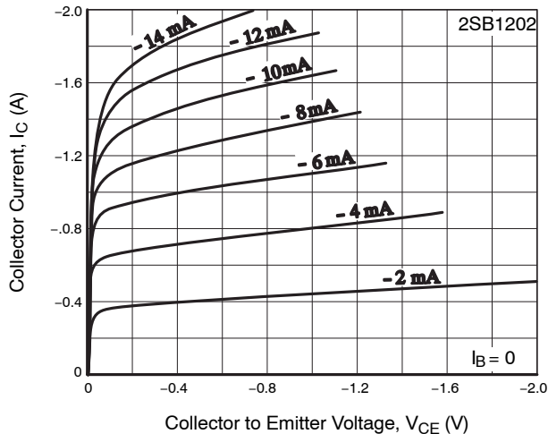
Figure 3. I_C - V_{CE}
