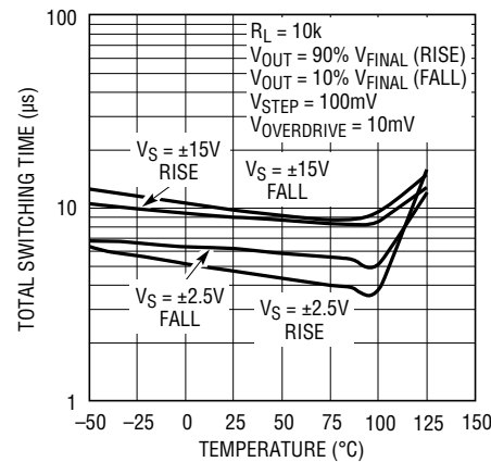
Total Switching Time vs Temperature
