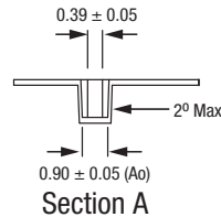
Section A
