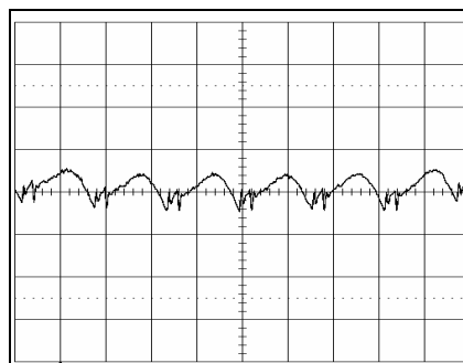
Output voltage ripple at: T_{ref} = +25^\circ\text{C} , V_i = 12\text{ V} , I_o = 10\text{ A} resistive load. Trace: output voltage (20 mV/div.). Time scale: (2 \mu\text{s} /div.).
