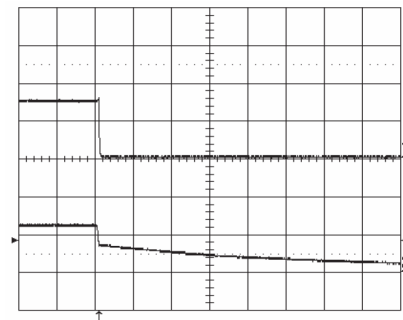
Shut-down enabled by disconnecting V_i at: T_{ref} = +25^\circ\text{C} , V_i = 12\text{ V} , I_o = 10\text{ A} resistive load. Top trace: output voltage (1.0 V/div.). Bottom trace: input voltage (10 V/div.). Time scale: (2 ms/div.).
