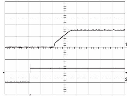
Start-up enabled by connecting V_i at: T_{ref} = +25^\circ\text{C} , V_i = 12\text{ V} , I_o = 10\text{ A} resistive load. Top trace: output voltage (1.0 V/div.). Bottom trace: input voltage (10 V/div.). Time scale: (2 ms/div.).
