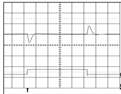
Output voltage response to load current step- change (2.5-7.5-2.5 A) at: T_{ref} = +25^\circ\text{C} , V_i = 12\text{ V} . Top trace: output voltage (100 mV/div.). Bottom trace: load current (10 A/div.). Time scale: (0.1 ms/div.).
