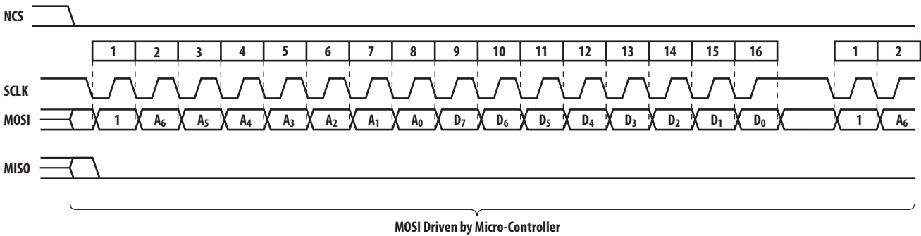
Figure 13. Write Operation
