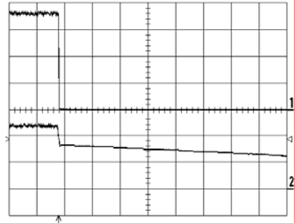
Shut-down enabled by disconnecting V_i at: T_{ref} = +25^\circ\text{C} , I_O = 26\text{ A} resistive load, V_i = 12.0\text{ V} . Top trace: output voltage (0.5 V/div.). Bottom trace: input voltage (5 V/div.). Time scale: 10.0 ms/div.
