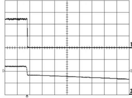
Shut-down enabled by disconnecting V_i at: T_{ref} = +25^{\circ}C , I_O = 26 A resistive load, V_i = 12.0 V. Top trace: output voltage (0.5 V/div.). Bottom trace: input voltage (5 V/div.). Time scale: 10.0 ms/div.
