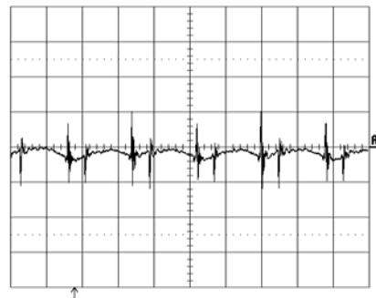
Output voltage ripple (20mV/div.) at: T_{ref} = +25^\circ\text{C} , I_O = 26\text{ A} resistive load, V_i = 12.0\text{ V} . Time scale: 1 \mu\text{s} /div. See the filter in the Output ripple and noise section (EMC Specification).
