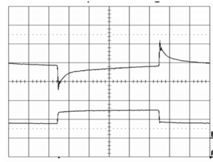
Output voltage response to load current step- change (13-26-13 A) at: T_{ref} = +25^\circ\text{C} , V_i = 12.0\text{ V} . Top trace: output voltage (100mV/div.). Bottom trace: load current (20 A/div.). Time scale: 0.1 ms/div.
