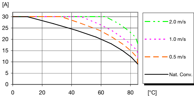
Available load current vs. ambient air temperature and airflow at V_I = 12.0 V, V_{OUT} = 3.3 V . See Thermal Consideration section.
