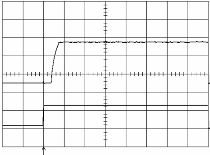
Start-up enabled by connecting V_i at: T_{ref} = +25^{\circ}C , I_O = 26 A resistive load, V_i = 12.0 V. Top trace: output voltage (0.5 V/div.). Bottom trace: input voltage (10 V/div.). Time scale: 10 ms/div.
