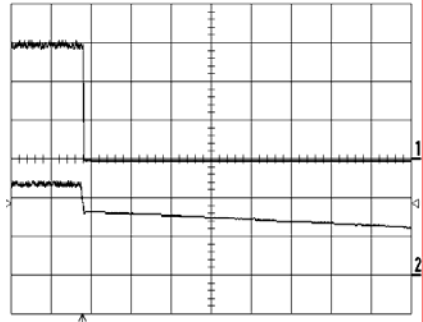
Shut-down enabled by disconnecting V_i at: T_{ref} = +25^\circ\text{C} , I_O = 26\text{ A} resistive load, V_i = 12.0\text{ V} . Top trace: output voltage (0.5 V/div.). Bottom trace: input voltage (5 V/div.). Time scale: 10.0 ms/div.
