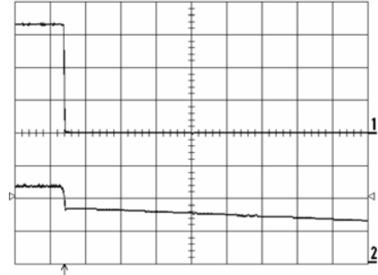
Shut-down enabled by disconnecting V_i at: T_{ref} = +25^\circ\text{C} , I_O = 26\text{ A} resistive load, V_i = 12.0\text{ V} . Top trace: output voltage (1.0 V/div.). Bottom trace: input voltage (5 V/div.). Time scale: 10.0 ms/div.
