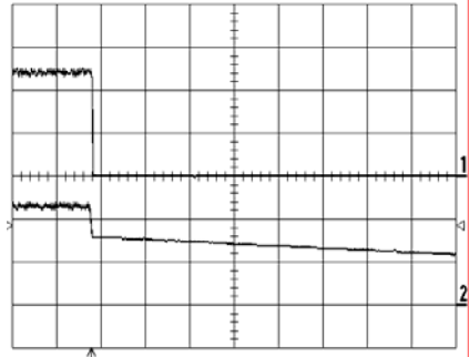
Shut-down enabled by disconnecting V_i at: T_{ref} = +25^{\circ}C , I_O = 26 A resistive load, V_i = 12.0 V. Top trace: output voltage (0.5 V/div.). Bottom trace: input voltage (5 V/div.). Time scale: 10.0 ms/div.
