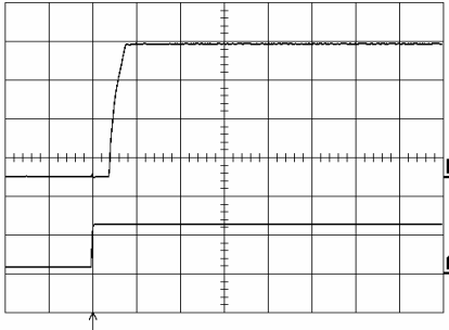
Start-up enabled by connecting V_i at: T_{ref} = +25^\circ\text{C} , I_O = 26\text{ A} resistive load, V_i = 12.0\text{ V} . Top trace: output voltage (0.5 V/div.). Bottom trace: input voltage (10 V/div.). Time scale: 10 ms/div.
