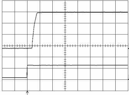
Start-up enabled by connecting V_i at: T_{ref} = +25^\circ\text{C} , I_O = 26\text{ A} resistive load, V_i = 12.0\text{ V} . Top trace: output voltage (1.0 V/div.). Bottom trace: input voltage (10 V/div.). Time scale: 10 ms/div.
