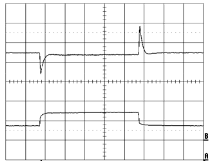
Output voltage response to load current step- change (13-26-13 A) at: T_{ref} = +25^{\circ}C , V_i = 12.0 V. Top trace: output voltage (100mV/div.). Bottom trace: load current (20 A/div.). Time scale: 0.1 ms/div.
