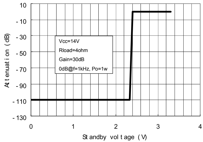
Figure 18. Attenuation vs. voltage on pin STBY
