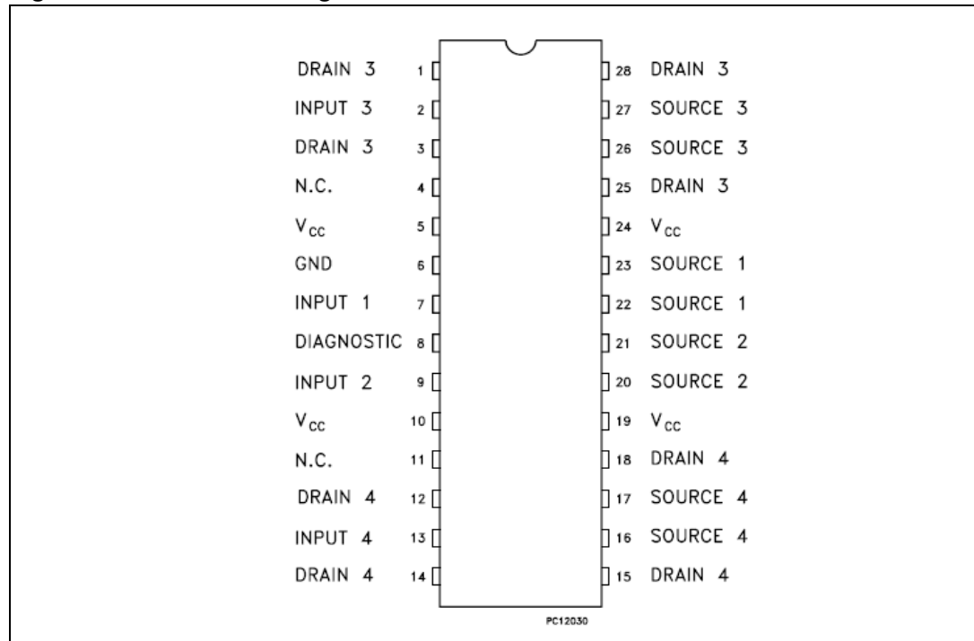
Figure 2. Connection diagram
