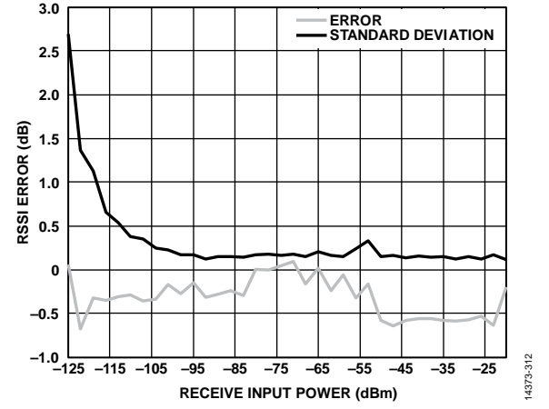
Figure 12. Packet RSSI Error vs. Rx Input Power with One-Point Calibration at -50 dBm, V_{DD} = 3.0\text{ V} , T_A = 25^\circ\text{C} , Configuration 169.43125 MHz/2.4 kbps (Error is Based on the Mean RSSI of 100 Packets)
