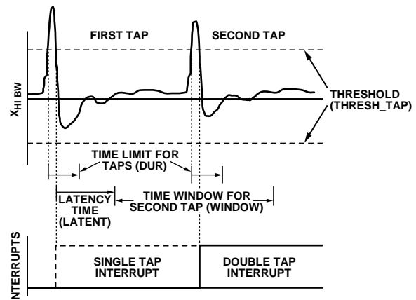
Figure 36. Tap Interrupt Function with Valid Single and Double Taps
