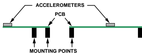
Figure 35. Incorrectly Placed Accelerometers
