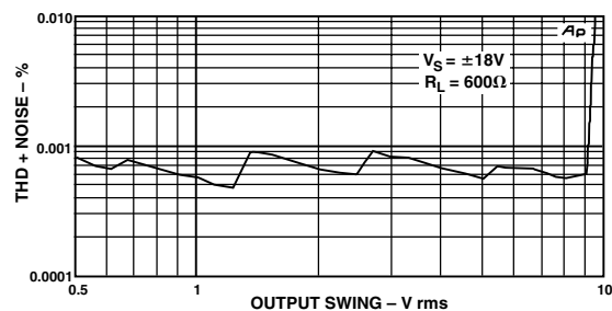
Figure 4. Headroom, THD + Noise vs. Output Amplitude (V rms); R_{LOAD} = 600 Ω, V_{SUP} = \pm 18 V
