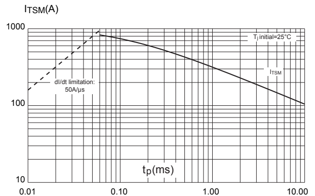
Figure 7. Non repetitive surge peak on-state current versus sinusoidal pulse width ( t_p < 10\text{ ms} )
