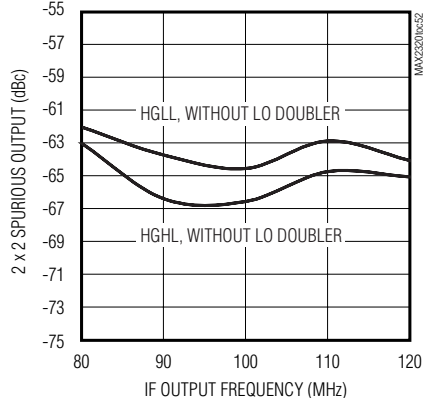
PCS-BAND MIXER 2 x 2 SPURIOUS REJECTION
