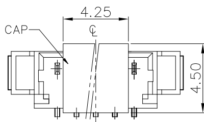
ASSEMBLY CAP
